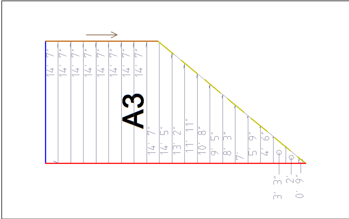
Plane A3 - 285.36 Sq. Ft.
