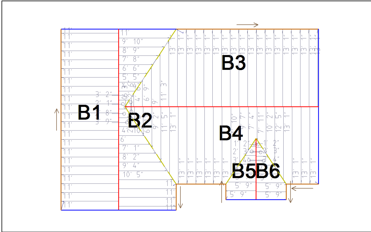
Section B - SS16, Standing Seam, PVDF, 24 Ga. Surface Area = 1180.24 Sq. Ft.
