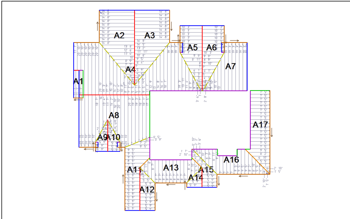
Section A - SS16, Standing Seam, PVDF, 24 Ga. Surface Area = 3207.33 Sq. Ft.
