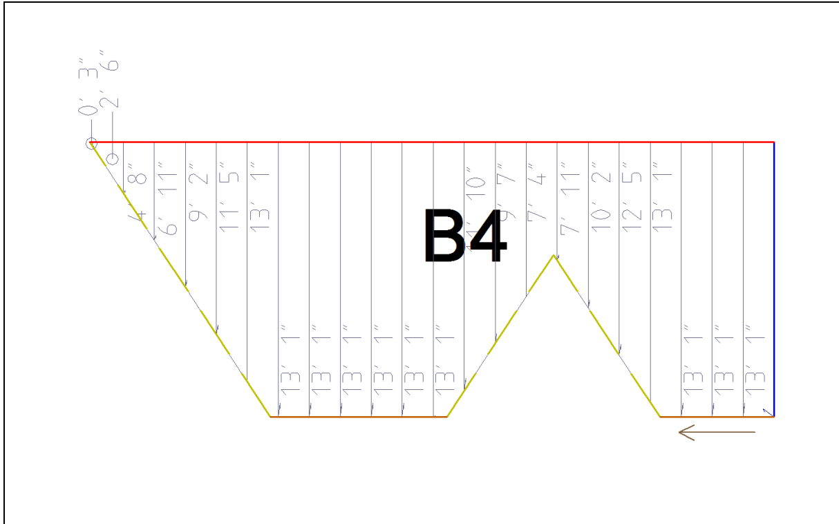
Plane B4 - 298.11 Sq. Ft.
