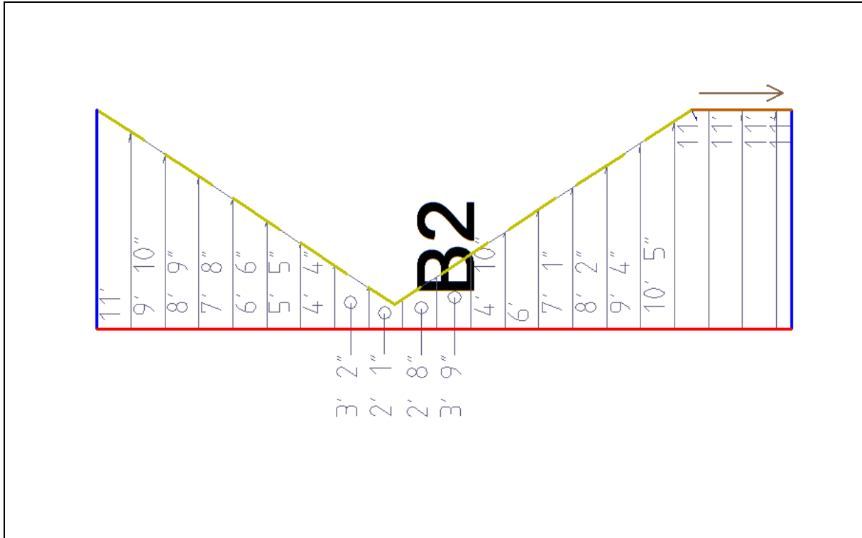
Plane B2 - 184.62 Sq. Ft.
