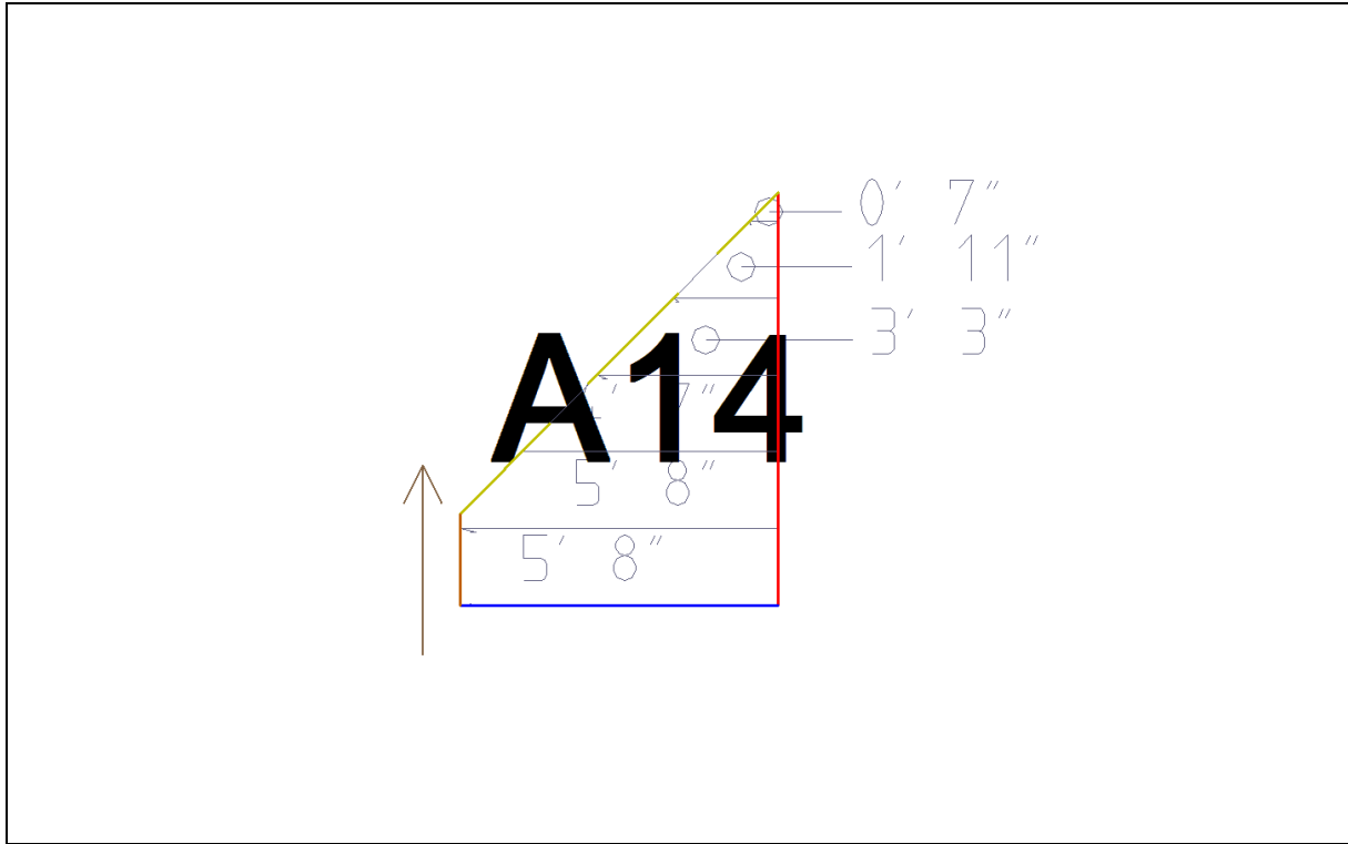
Plane A14 - 24.76 Sq. Ft.
