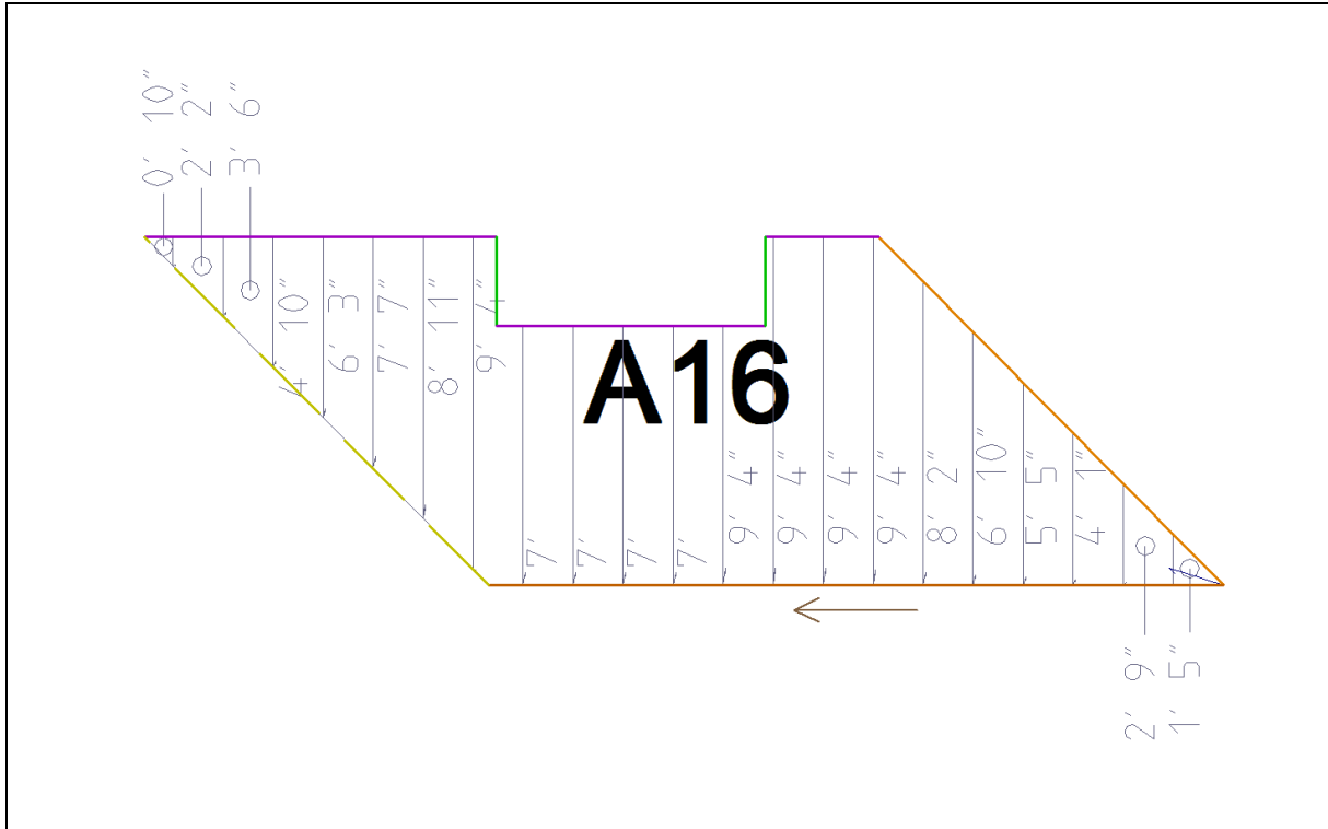
Plane A16 - 165.33 Sq. Ft.
