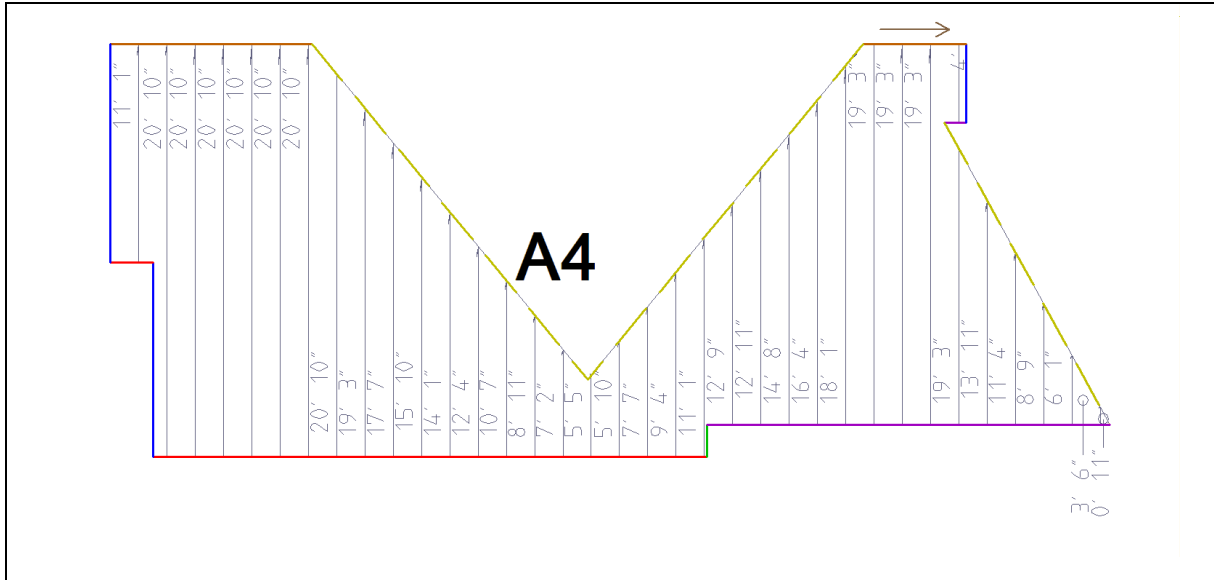
Plane A4 - 622.44 Sq. Ft.
