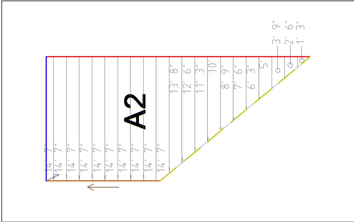
Plane A2 - 285.36 Sq. Ft.
