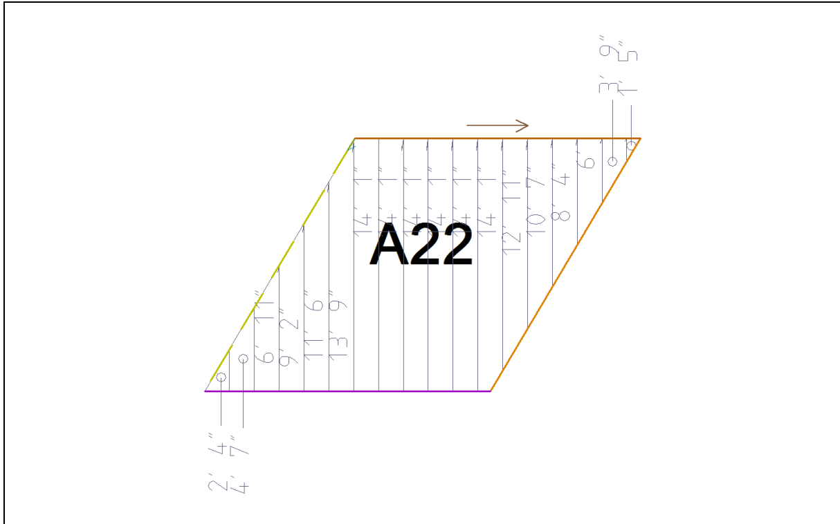
Plane A22 - 212.20 Sq. Ft.
