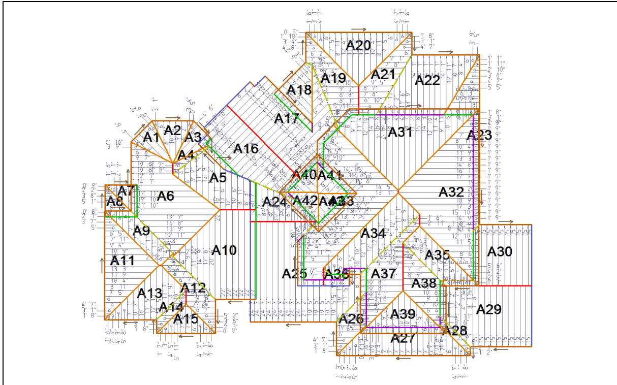
Section A - SS NAIL STRIP, Standing Seam, PVDF, 24 Ga. Surface Area = 5940.28 Sq. Ft.
