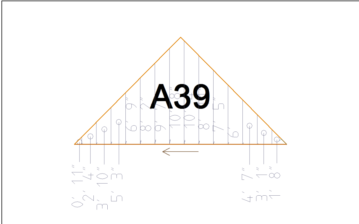
Plane A39 - 101.23 Sq. Ft.
