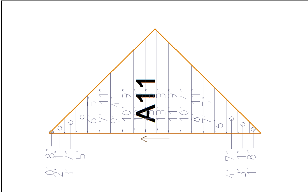
Plane A11 - 161.46 Sq. Ft.
